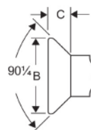
COUNTERSUNK HEAD
